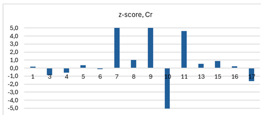
Figure 4.7. Z-scores of the laboratories for freshwater Cr, sample A and B. Laboratory code no. 7 (Z-score 28.4), 9 (Z-score 12.2) and 10 (Z-score -8.2) are outside the range of the figure.
