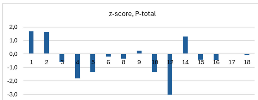
Figure 4.17. Z-scores of the laboratories for wastewater P-total, sample A and B. Laboratory code no. 12 (z-score -14.1) is outside the range of the figure.
