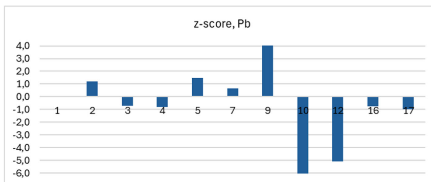
Figure 4.22. Z-scores of the laboratories for wastewater Pb, sample A and B. Laboratory code no. 9 (z-score 33.4) and 10 (z-score -7.1) are outside the range of the figure.
