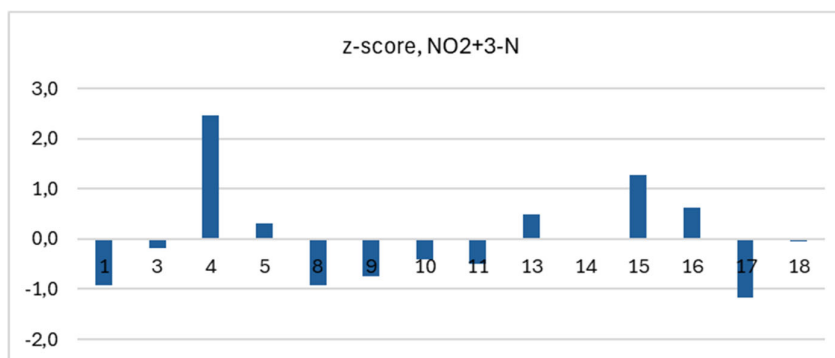
Figure 4.2. Z-scores of the laboratories for freshwater NO 2+3 -N, sample A and B.
