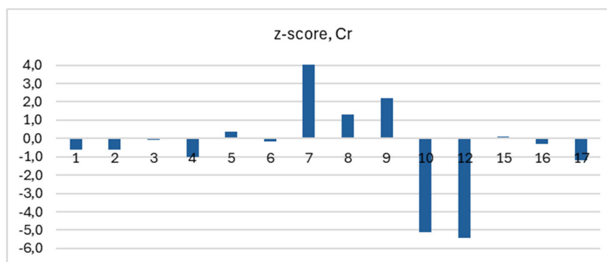
Figure 4.19. Z-scores of the laboratories for wastewater Cr, sample A and B. Laboratory code no. 7 (z-score 10,7) is outside the range of the figure.
