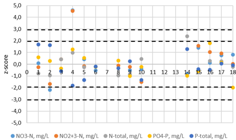
Figure 5.3. z-score results for wastewater, nutrients: z < |2| : 61 results; |3| < z < |2| : 2 results; z > |3| : 6 results. Four z-score not shown (lab 12: NO 3 -N, NO 2+3 , N-total, and P-total). The laboratory code numbers are on the x-axis. The dotted lines represent z = |2| and z = |3| . Lab 7, 11 and 13 did not analyse nutrients in wastewater.
