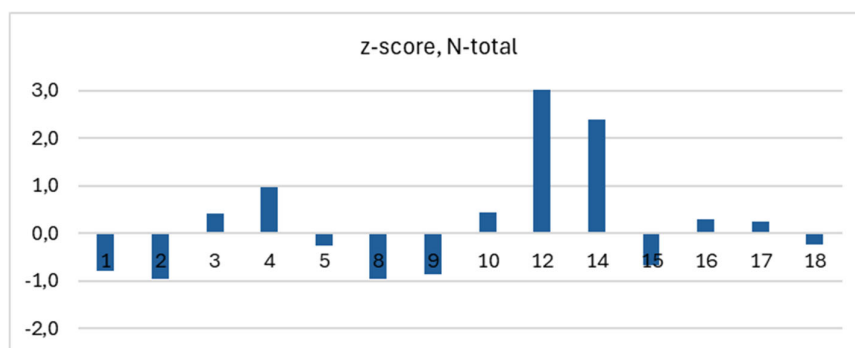
Figure 4.15. Z-scores of the laboratories for wastewater N-total, sample A and B. Laboratory code no. 12 (z-score 1029) is outside the range of the figure.
