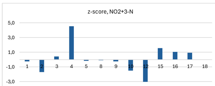
Figure 4.14. Z-scores of the laboratories for wastewater NO 2+3 -N, sample A and B. Laboratory code no. 12 (z-score -33.7) is outside the range of the figure.
