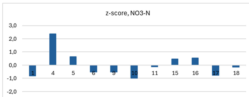
Figure 4.1. Z-scores of the laboratories for freshwater NO 3 -N, sample A and B.
