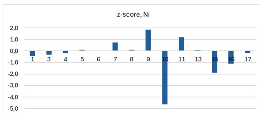
Figure 4.9. Z-scores of the laboratories for freshwater Ni, sample A and B.
