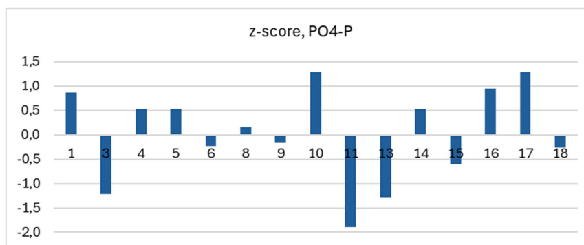
Figure 4.4. Z-scores of the laboratories for freshwater PO 4 -P, sample A and B.
