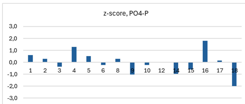
Figure 4.16. Z-scores of the laboratories for wastewater PO 4 -P, sample A and B.
