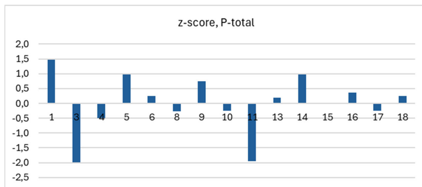
Figure 4.5. Z-scores of the laboratories for freshwater P-total, sample A and B.
