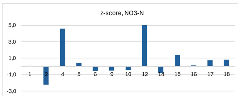
Figure 4.13. Z-scores of the laboratories for wastewater NO 3 -N, sample A and B. Laboratory code no. 12 (z-score 4114) is outside the range of the figure.
