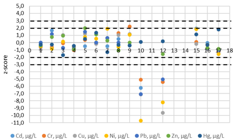
Figure 5.4. z-score results for wastewater, metals: z < |2| : 81 results; |3| < z < |2| : 1 result; z > |3| : 11 results. Three z-scores not shown (lab 7: 10.7 for Cr; lab 9: 33.4 for Pb; lab 10: -12.6 for Zn). The laboratory code numbers are on the x-axis. The dotted lines represent z = |2| and z = |3| . Lab 11, 13 and 18 did not analyse metals in Wastewater.
