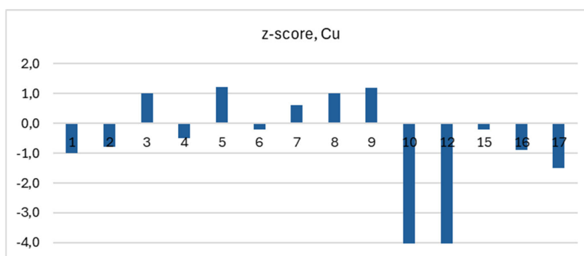
Figure 4.20. Z-scores of the laboratories for wastewater Cu, sample A and B. Laboratory code no. 10 (z-score -7.1) and 12 (z-score -9.6) are outside the range of the figure.
