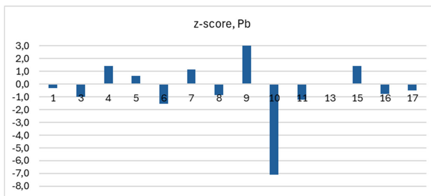
Figure 4.10. Z-scores of the laboratories for freshwater Pb, sample A and B. Laboratory code no. 9 (Z-score 54.1) is outside the range of the figure.
