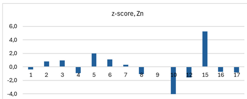
Figure 4.23. Z-scores of the laboratories for wastewater Zn, sample A and B. Laboratory code no. 10 (z-score -12.6) is outside the range of the figure.
