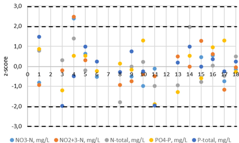
Figure 5.1. z-score results for freshwater A/B samples, nutrients: z < |2| : 67 results; |3| < z < |2| : 2 results; z > |3| : 0 result. The laboratory code numbers are on the x-axis. The dotted lines represent z = |2| and z = |3| . Lab. 2, 7 and 12 did not analyse nutrients in freshwater.
