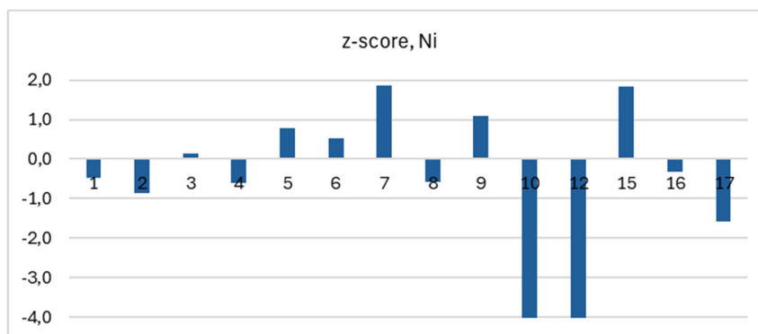
Figure 4.21. Z-scores of the laboratories for wastewater Ni, sample A and B. Laboratory code no. 10 (z-score -10.7) and 12 (z-score -8.2) are outside the range of the figure.
