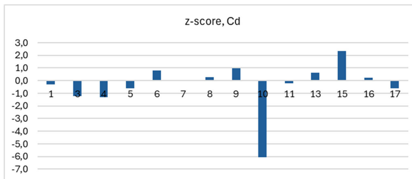
Figure 4.6. Z-scores of the laboratories for freshwater Cd, sample A and B.
