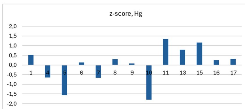
Figure 4.12. Z-scores of the laboratories for freshwater Hg, sample A and B.
