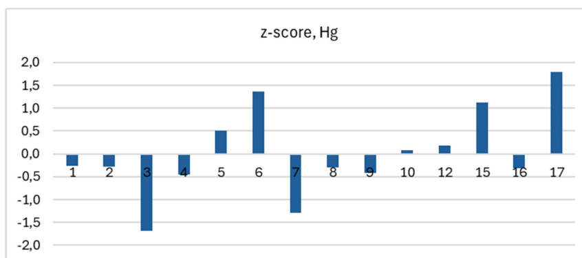
Figure 4.24. Z-scores of the laboratories for wastewater Hg, sample A and B.
