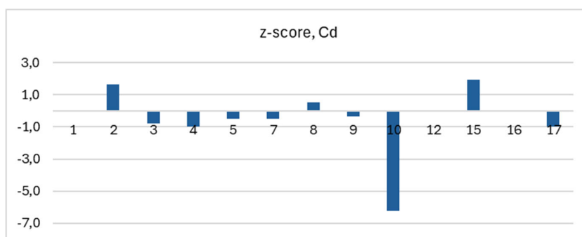
Figure 4.18. Z-scores of the laboratories for wastewater Cd, sample A and B.
