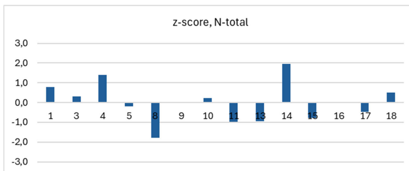
Figure 4.3. Z-scores of the laboratories for freshwater N-total, sample A and B..
