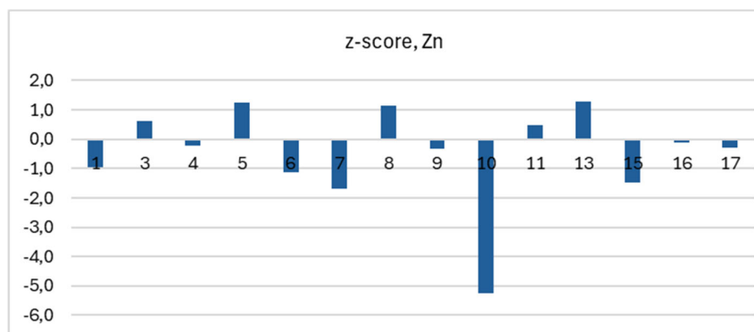
Figure 4.11. Z-scores of the laboratories for freshwater Zn, sample A and B.
