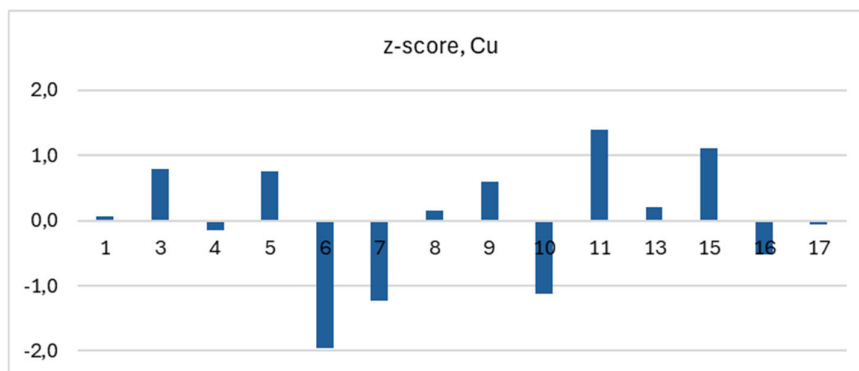
Figure 4.8. Z-scores of the laboratories for freshwater Cu, sample A and B.
