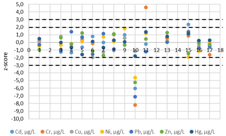
Figure 5.2. z-score results for freshwater, metals: z < |2| : 91 results; |3| < z < |2| : 1 result; z > |3| : 5 results. Three z-score not shown (lab 7: 28.4 for Cr: and lab. 9: 12.2 for Cr and 54.1 for Pb). The laboratory code numbers are on the x-axis. The dotted lines represent z = |2| and z = |3| . Lab. 2, 12, 14 and 18 did not analyse metals in freshwater.
