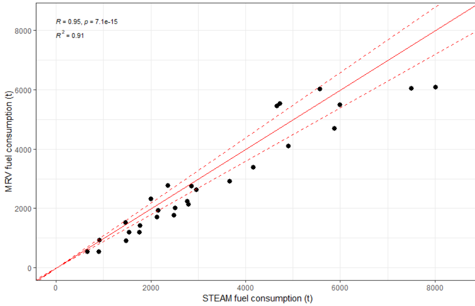
Figure 15 Scatterplot of total annual fuel consumed between STEAM (x-axis) and MRV (y-axis) of bulk carriers. The solid red line indicates 100% correlation between STEAM and MRV and the dashed lines a 10% deviation from perfect correlation. Correlation (R) and goodness of fit (R 2 ) of linear regression in the top left corner.
