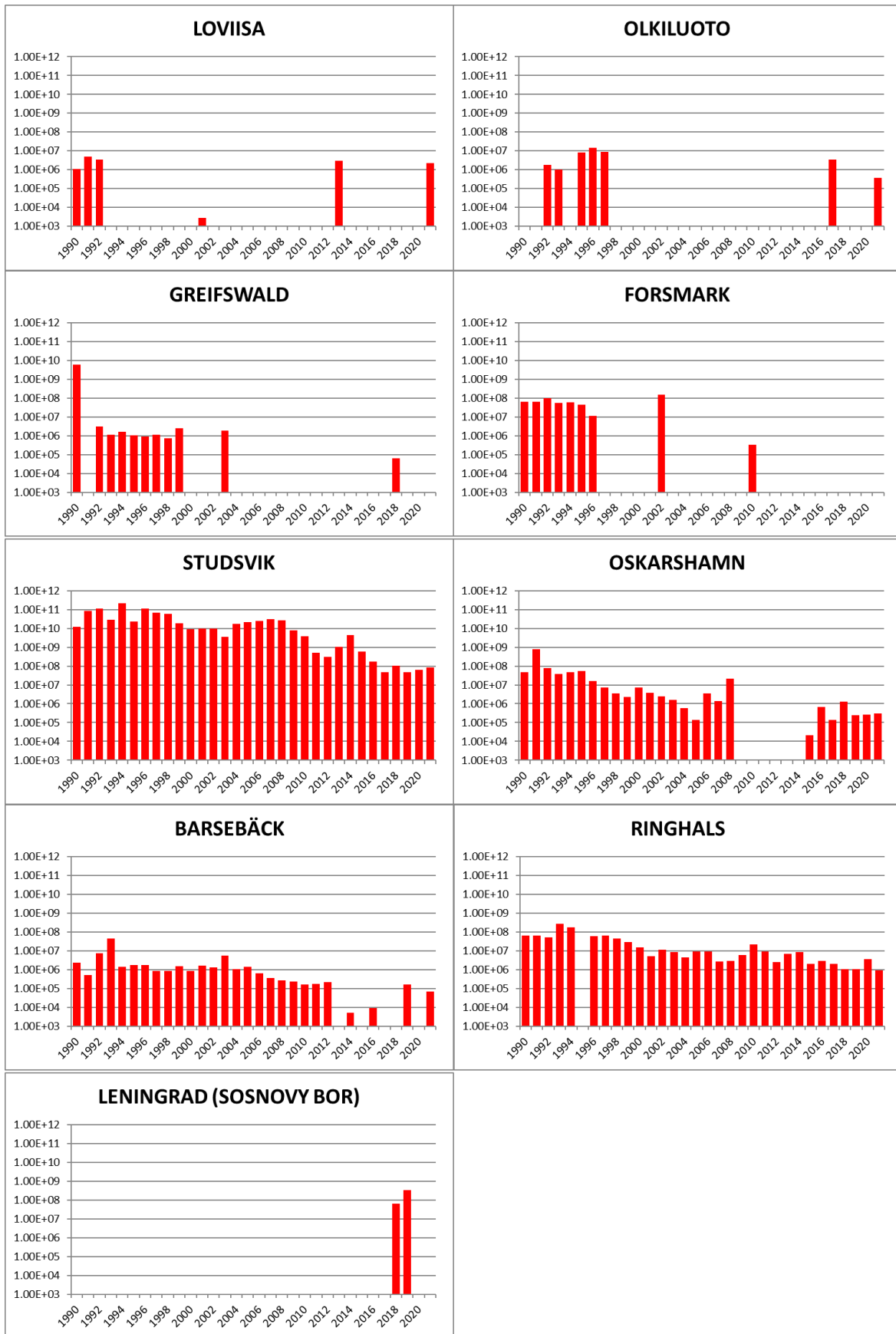
Fig. 2. Annual liquid discharges of strontium-90 from nuclear power plants and other nuclear facilities into the Baltic Sea in 1990-2021 (Note: logarithmic scales in the graphs).
