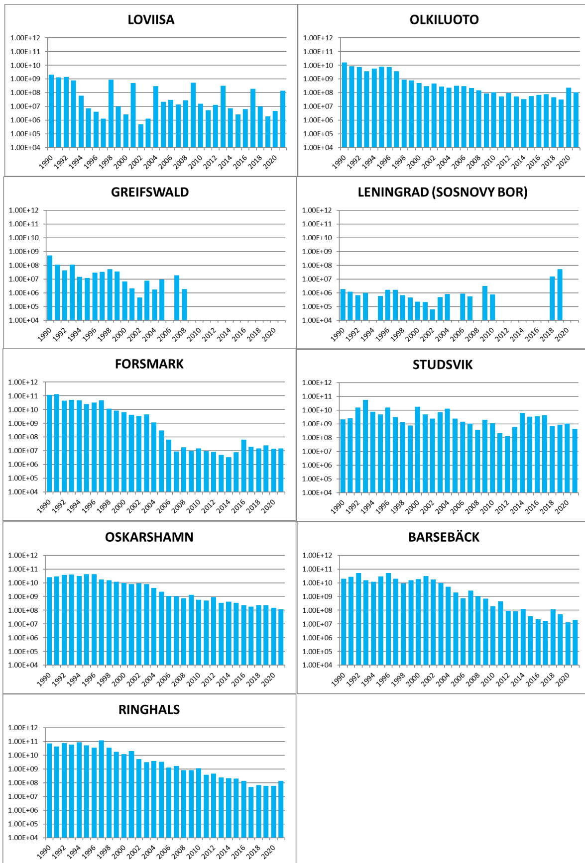
Fig. 3. Annual liquid discharges of cobalt-60 from nuclear power plants and other nuclear facilities into the Baltic Sea in 1990-2021 (Note: logarithmic scales in the graphs).
