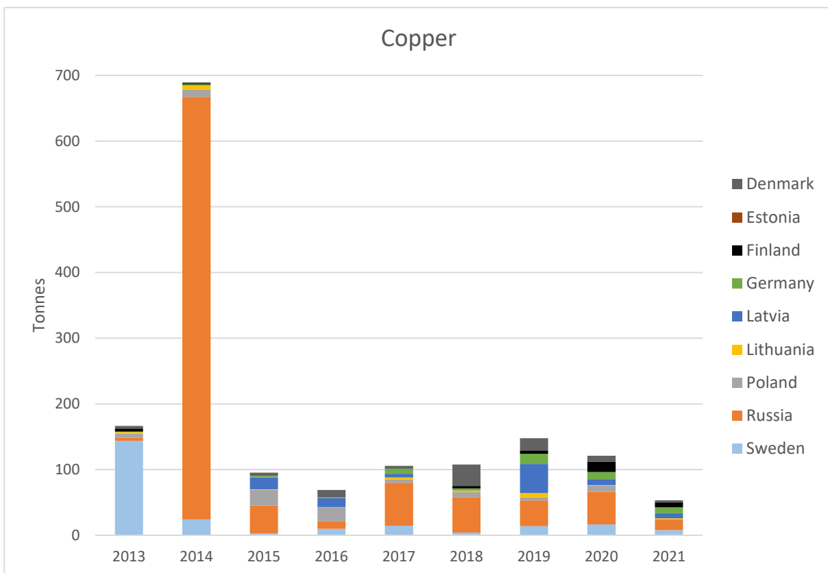
Figure 37. Total amount of copper in dredged material deposited at sea in 2013-2021.
