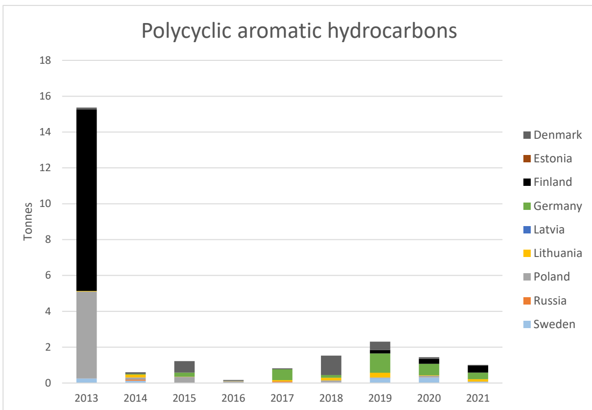
Figure 39. Total amount of polycyclic aromatic hydrocarbons in dredged material deposited at sea in 2013-2021.
