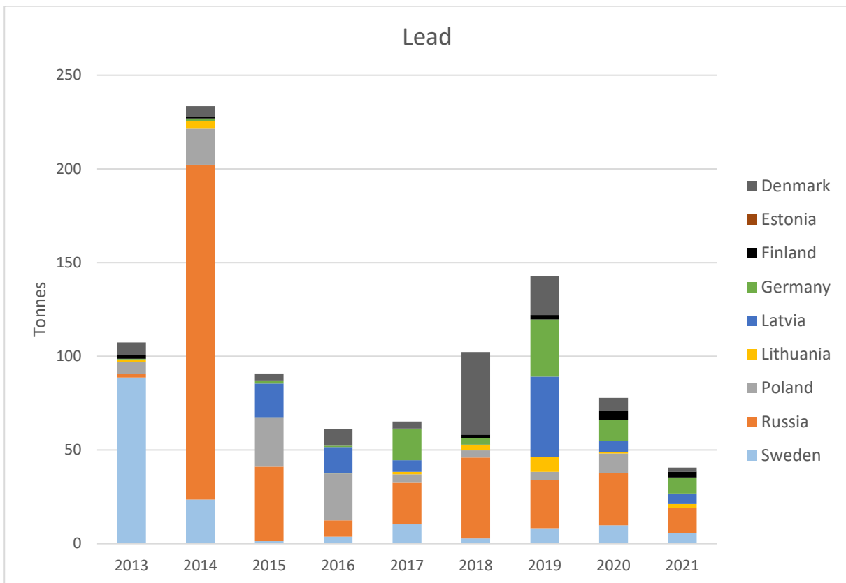
Figure 35. Total amount of lead in dredged material deposited at sea in 2013-2021.
