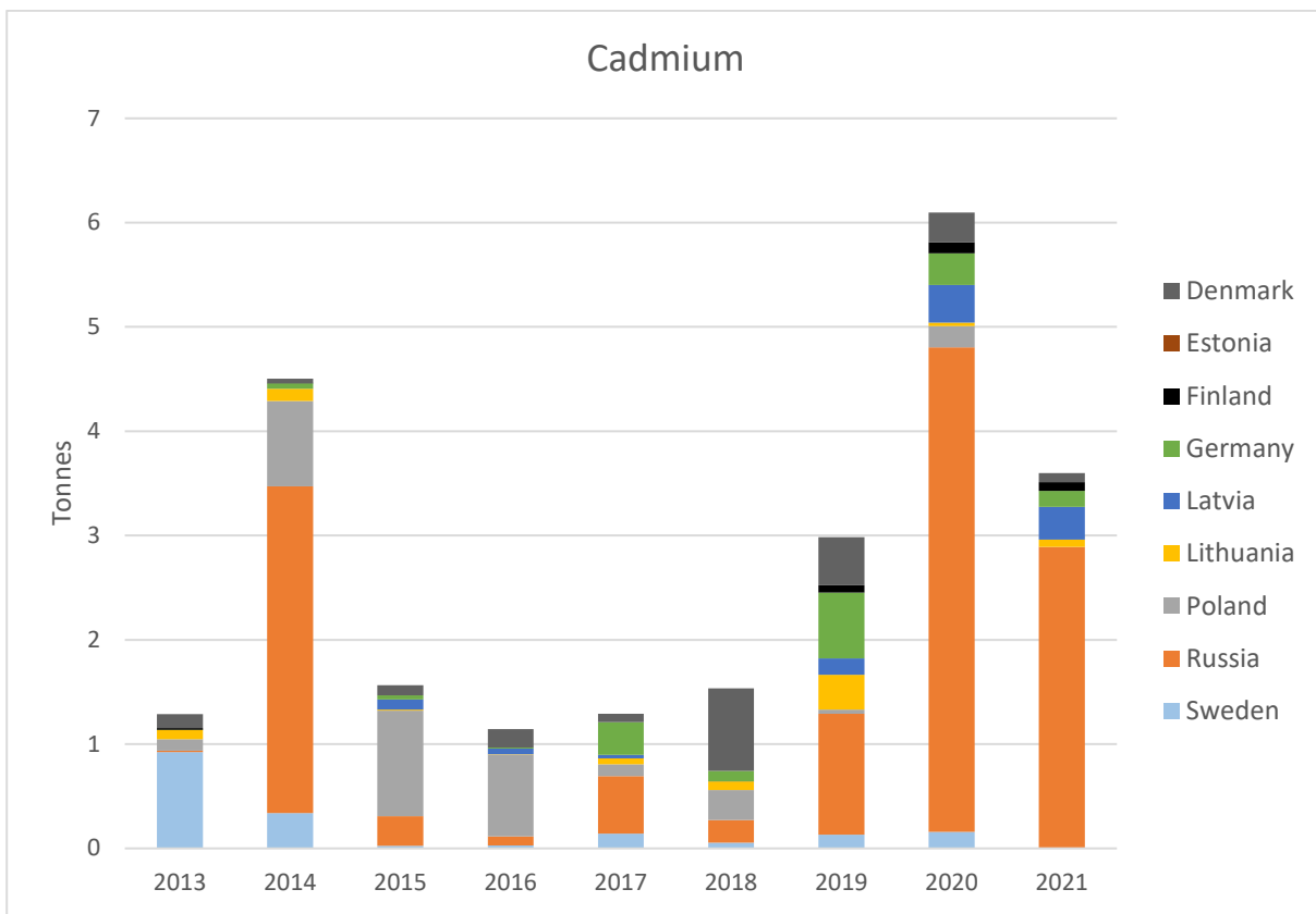
Figure 36. Total amount of cadmium in dredged material deposited at sea in 2013-2021.
