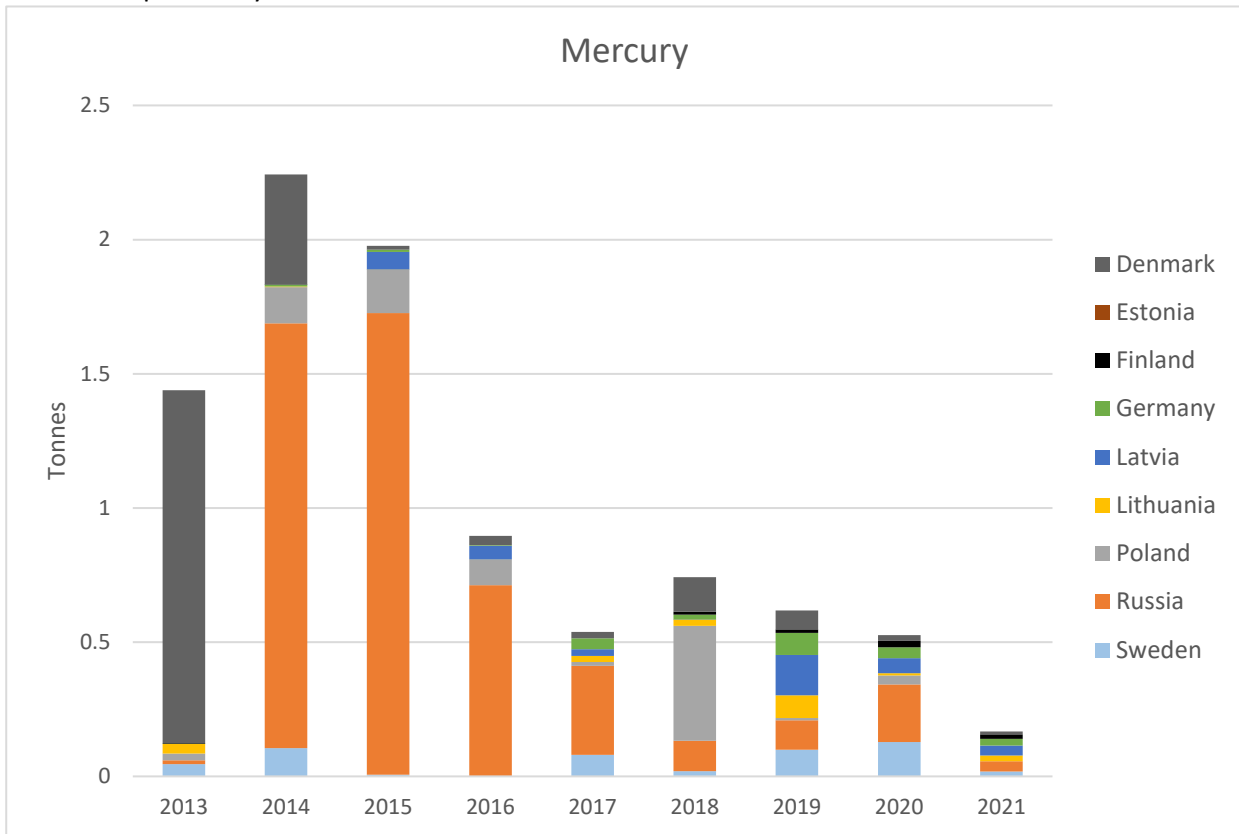
Figure 34. Total amount of mercury in dredged material deposited at sea in 2013-2021.
