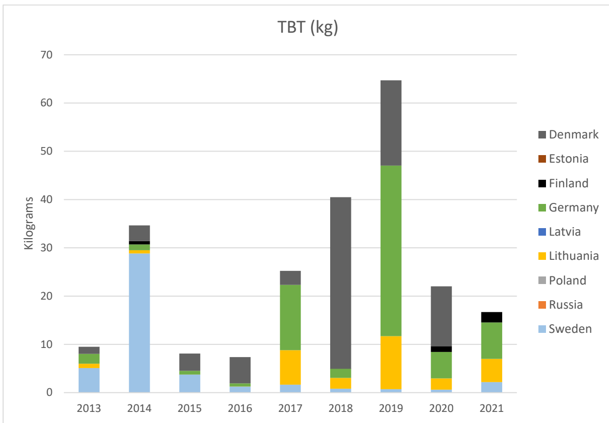
Figure 38. Total amount of TBT in dredged material deposited at sea in 2013-2021.
