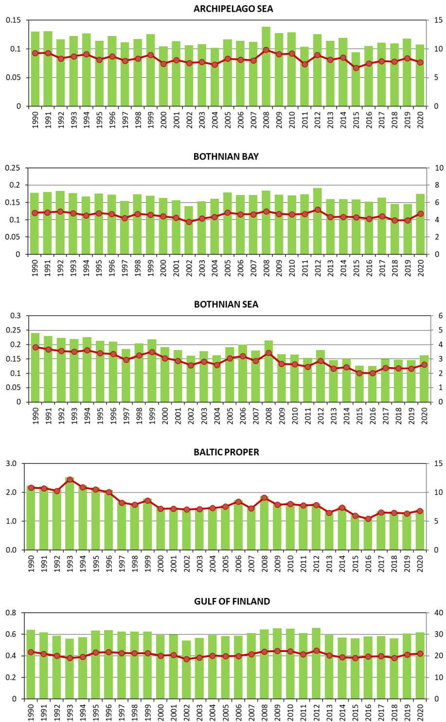
Figure 2. Time-series of computed total annual atmospheric deposition of B(a)P to nine sub-basins of the Baltic Sea for the period 1990-2020 in t\ y^{-1} as green bars (left axis) and total deposition fluxes in g\ km^{-2}\ y^{-1} as red lines (right axis).
