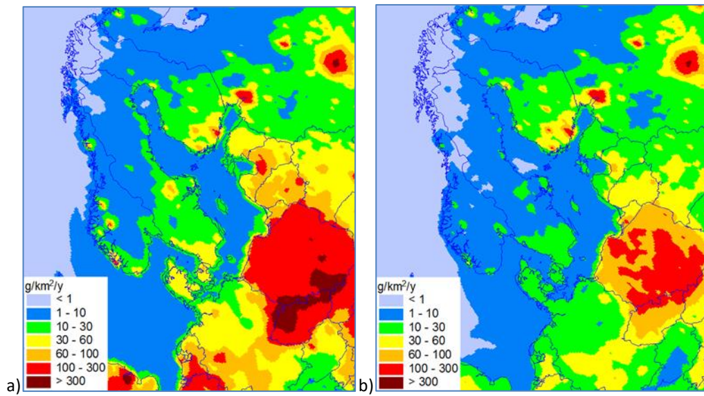
Figure 3. Spatial distribution of modelled annual total deposition fluxes of B(a)P in the Baltic Sea region for 1990 (a) and 2020 (b), \text{g km}^{-2} \text{y}^{-1} .
