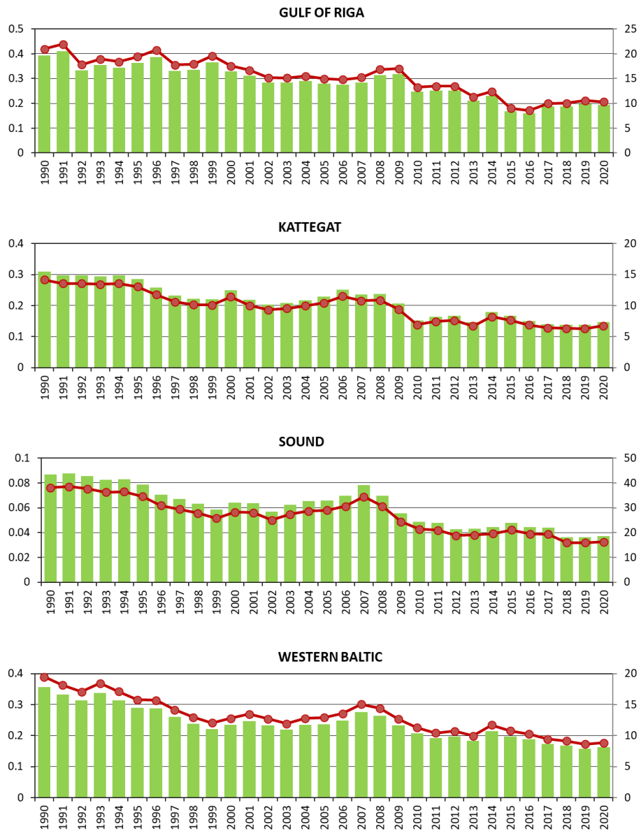
Figure 2. (continued). Time-series of computed total annual atmospheric deposition of B(a)P to nine sub-basins of the Baltic Sea for the period 1990-2020 in t\ y^{-1} as green bars (left axis) and total deposition fluxes in g\ km^{-2}\ y^{-1} as red lines (right axis).
