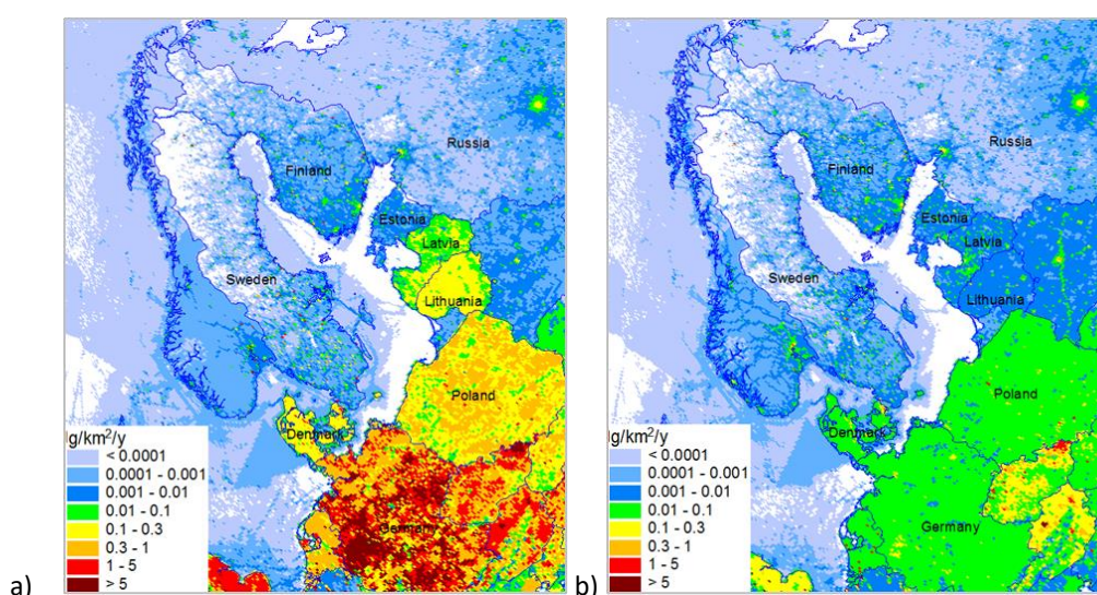
Figure 2. Spatial distribution of annual anthropogenic HCB emissions to the atmosphere in the Baltic Sea region in 1990 (a) and in 2019 (b), in g\ km^{-2}\ y^{-1} .
