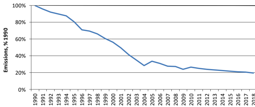
Figure 1. Total annual emissions of PCB-153 to air from HELCOM Contracting Parties in period 1990-2018 (% of 1990).
