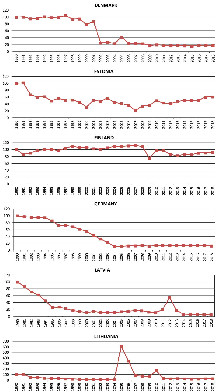
Figure 3. Trends in annual atmospheric emissions of PCB-153 from HELCOM Contracting Parties from 1990 to 2018, plotted as percentage of the 1990 value. Unit: %. The emission data of the CP refer to the total area of the CP except for Russia, where emissions from the territory of Russia within the EMEP domain is used.
