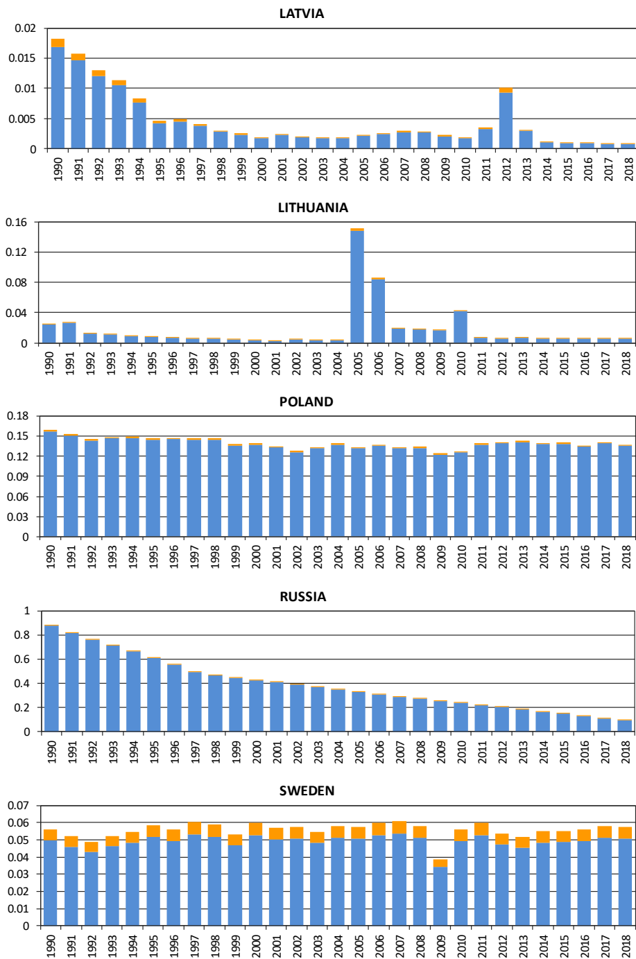
Figure 2. (continued). PCB-153 emissions of HELCOM Contracting Parties (CP) to air as totals in tonnes/year for the period 1990-2018. Orange sections of the bars identify the fraction of emission deposited to the Baltic Sea. The emission data of the CP refer to the total area of the CP except for Russian Federation, for which emissions from the territory of Russian Federation within the EMEP domain is used.
