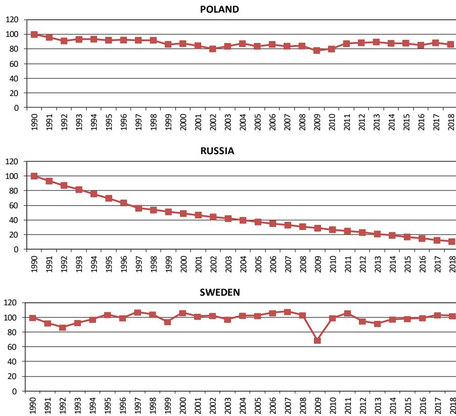
Figure 3. Trends in annual atmospheric emissions of PCB-153 from HELCOM Contracting Parties from 1990 to 2018, plotted as percentage of the 1990 value. Unit: %. The emission data of the CP refer to the total area of the CP except for Russia, where emissions from the territory of Russia within the EMEP domain is used.
