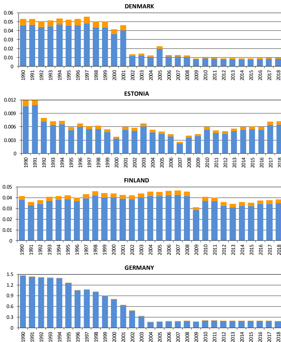
Figure 2. PCB-153 emissions of HELCOM Contracting Parties (CP) to air as totals in tonnes/year for the period 1990-2018. Orange sections of the bars identify the fraction of emission deposited to the Baltic Sea. The emission data of the CP refer to the total area of the CP except for Russian Federation, for which emissions from the territory of Russian Federation within the EMEP domain is used.
