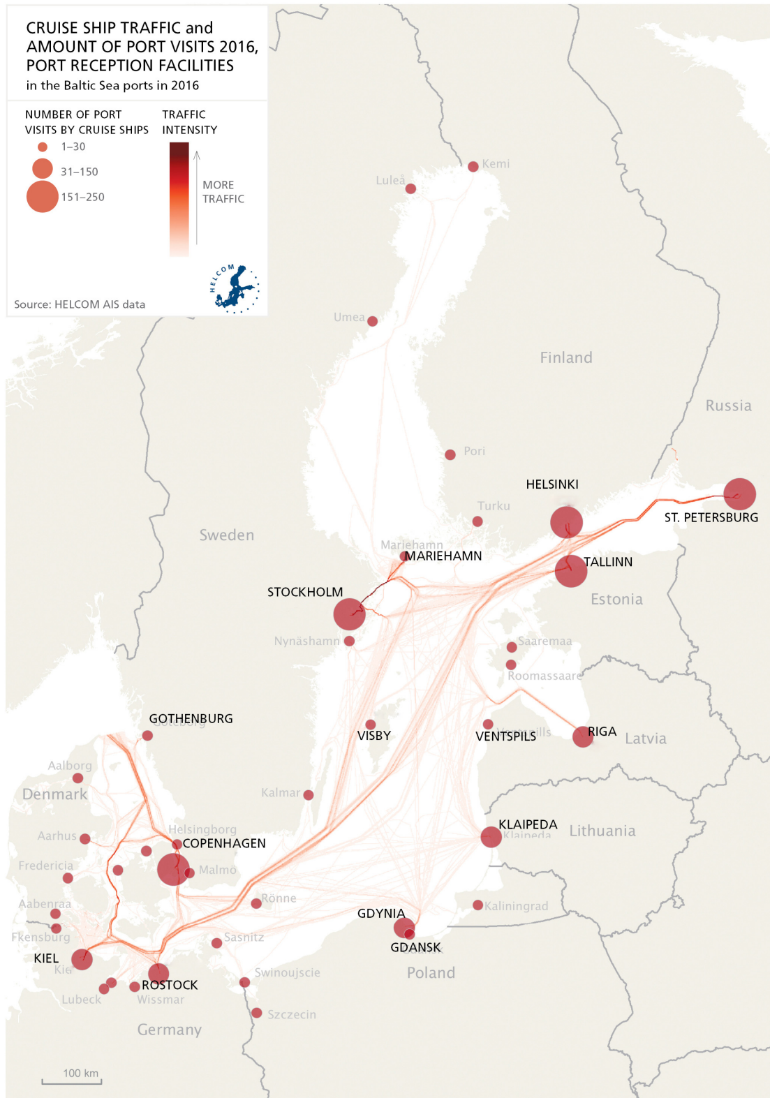
Figure. 4: Cruise ships traffic intensity and ports visits in 2016
