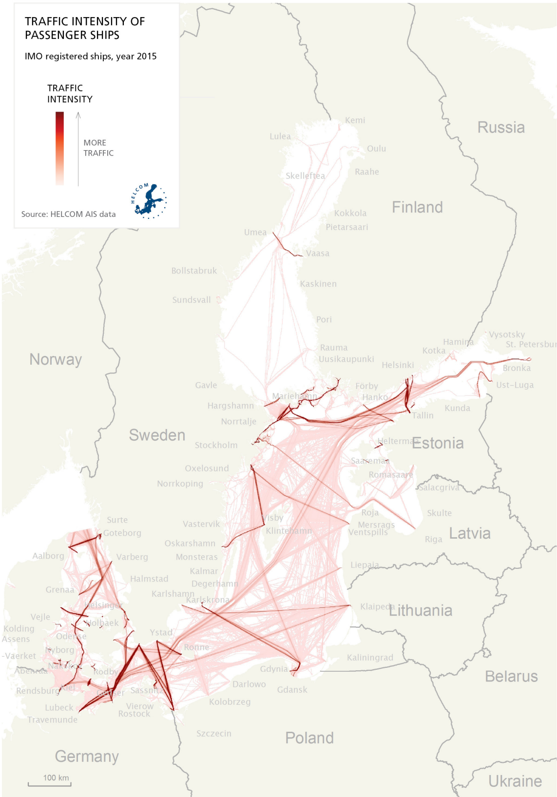
Figure. 2: Traffic intensity map of all passenger ships in the Baltic Sea region in 2015 The fleet of the passenger ships can be divided into smaller categories
