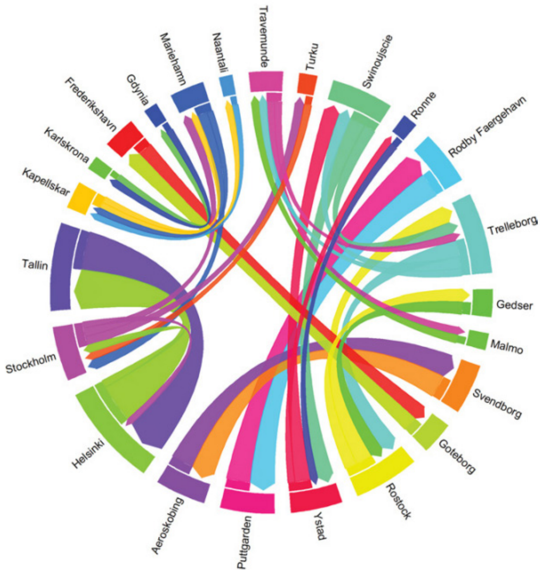
Figure 1: Passenger ship movements between ports (arrival and departures) in 2015 (between the 50 biggest ports and a minimum of 500 trips between ports) (Source: HELCOM, 2018).
