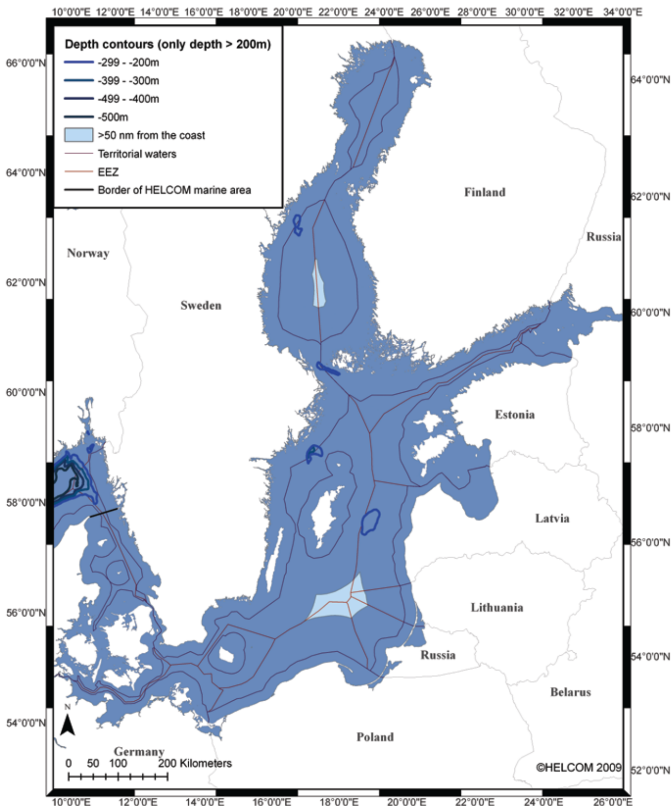
Map 9. Map of the Baltic Sea showing marine areas 50 nm from the nearest land and of the depth of 200 m and more.
