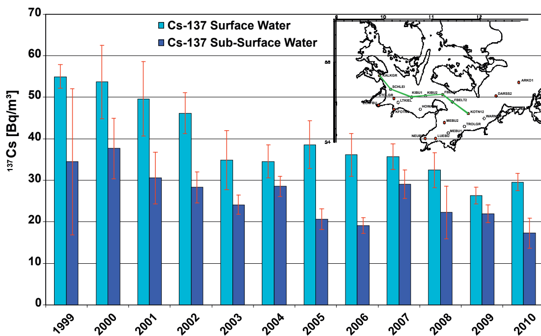
Figure 3a.3. Time series of ^{137}\text{Cs} mean concentrations from stations characterising the inflow of bottom water into the Western Baltic.
