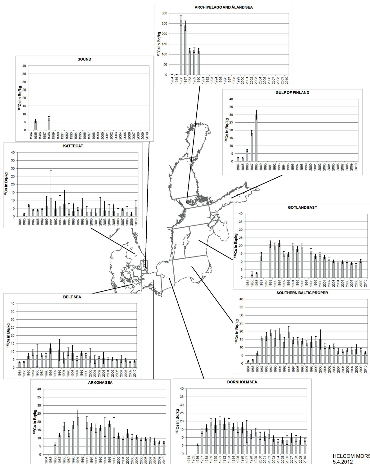
Figure 3c.2. Annual average ^{137}\text{Cs} concentrations (Bq/kg wet weight) in cod muscle (fillets) in 1984-2010. Uncertainty has been indicated as bar lines. NOTE: Variable scale in graphs.
