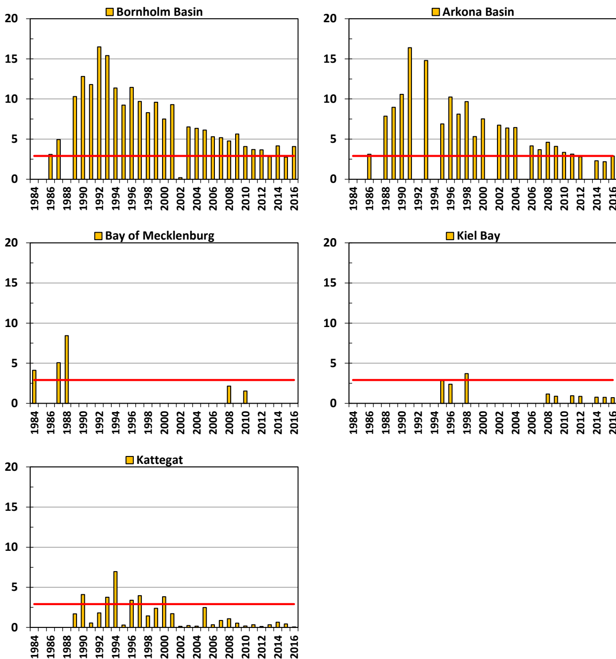
Results figure 2. ^{137}\text{Cs} concentrations (in \text{Bq kg}^{-1} ) in flatfish - plaice and flounder (whole fish without head and entrails, or flesh without bones) in 1984–2016, as annual means by sub-basin. Red line indicates the threshold value-2.9 \text{Bq kg}^{-1} calculated as average of pre-Chernobyl (1984–1985) concentrations.
