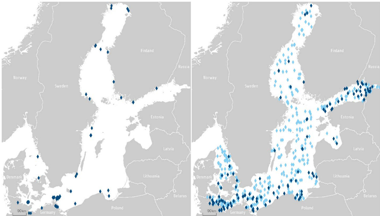
Optimal monitoring figure 1. Monitoring stations for biota (left) and seawater (right) used to assess trends in radioactive Cs-137. Dark blue symbols indicate data series incorporated into the specific assessment period 2011-2016 and pale blue symbols indicate those stations also within the overall assessment period presented. HELCOM scale 2 assessment units are used for this indicator.
