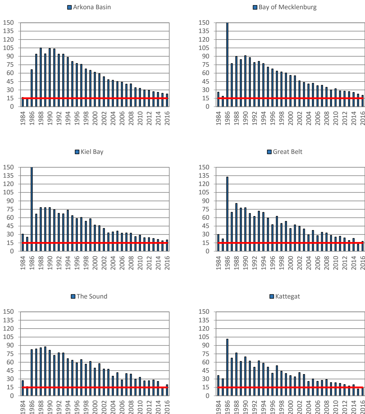
Results figure 3. 137 Cs concentrations (in Bq m -3 ) in seawater (sampling depth less than 10 m) in 1984-2016, as annual mean values by sub-basin. Red line indicates the threshold value (15 Bq m -3 ) calculated as average of pre-Chernobyl (1984-1985) concentrations.
