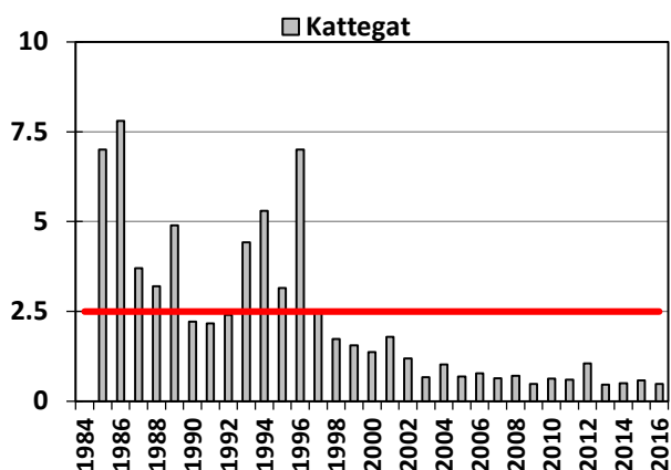
Results figure 1. 137 Cs mean concentrations (in Bq kg -1 wet weight) in herring (whole fish without head and entrails or flesh without bones) in 1984–2016, as annual mean by sub-basin. Red line indicates the good status boundary (threshold value 2.5 Bq kg -1 ) calculated as average of pre-Chernobyl (1984–1985) concentrations. Notice variable scale in graphs.
